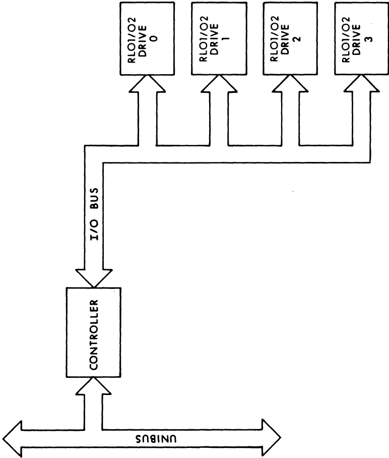
Figure 2-2 RL11/RL211 SYSTEM BLOCK DIAGRAM
