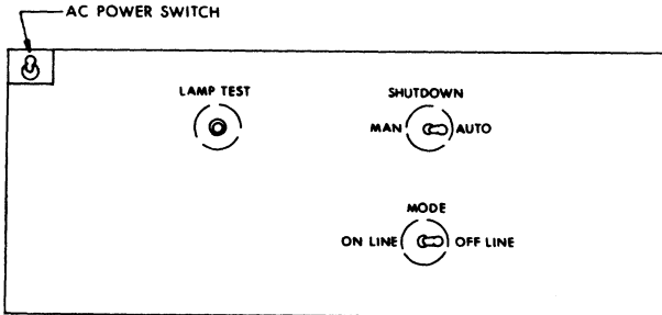
CR11, CR11-A REAR PANEL
