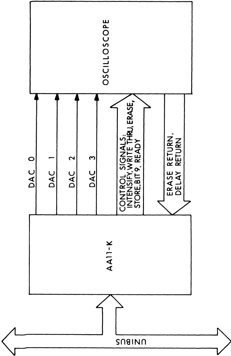
Figure 6-1 AA11-K BLOCK DIAGRAM
